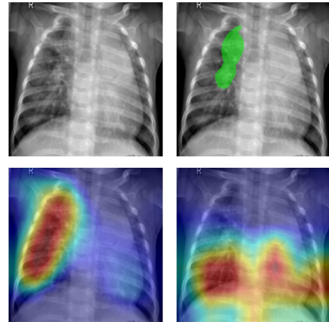
Figure 1: Saliency Map Example. Top row shows the original X-ray and a raw expert annotation. Bottom row displays CAM for VGG-16 (left) and ResNet-50 (right).
