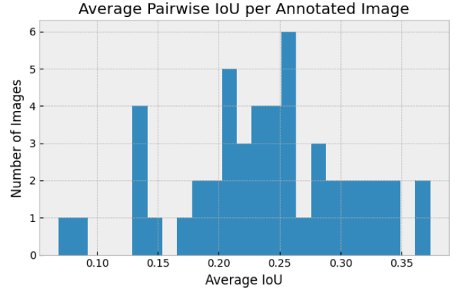
Figure 5: Average IoU. For each image, we measure the IoU between all pairs of annotations for that image and then compute the average.
