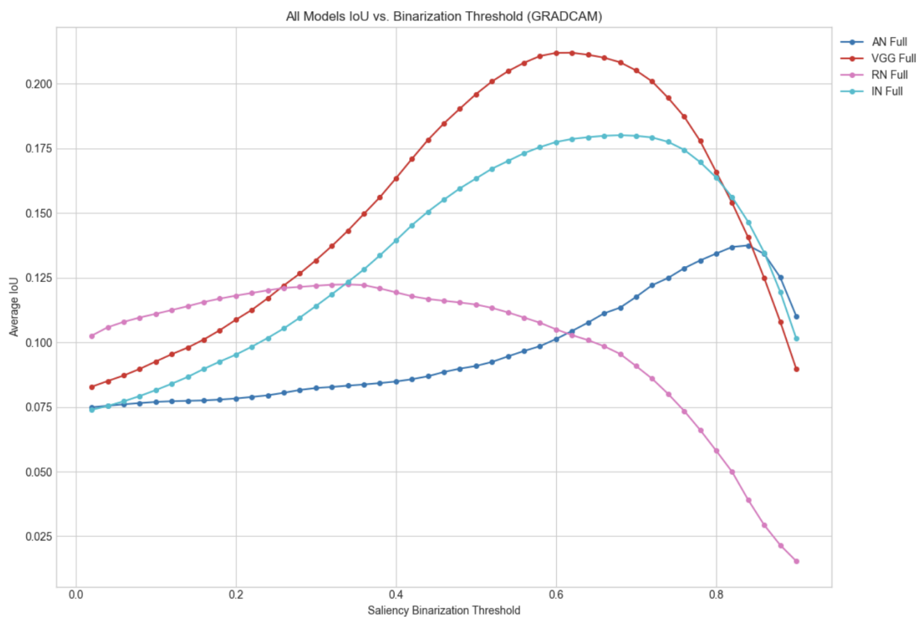
Figure 7: Model–Expert IoUs vs. Thresholds (Grad-CAM).
