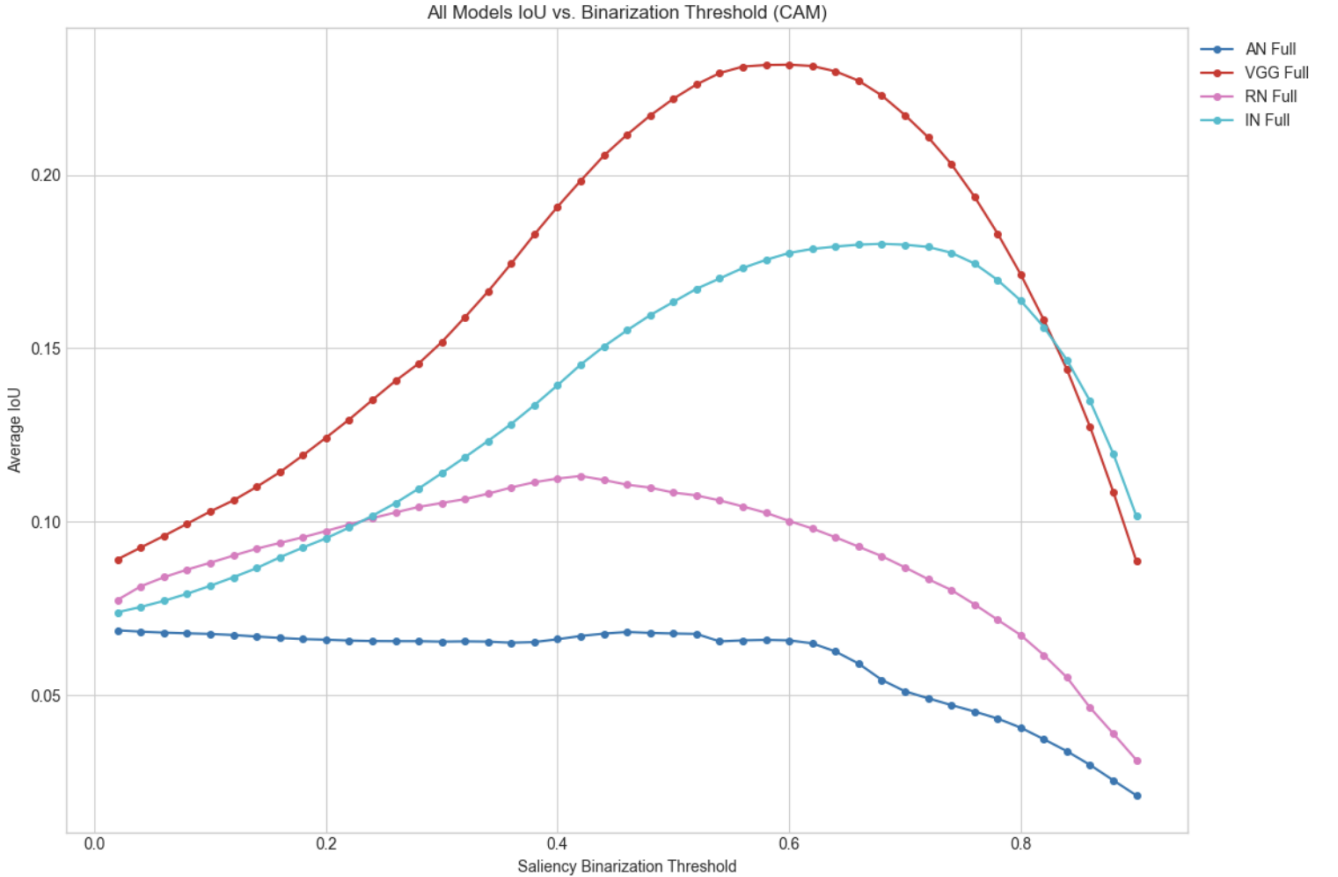
Figure 6: Model-Expert IoUs vs. Thresholds (CAM).
