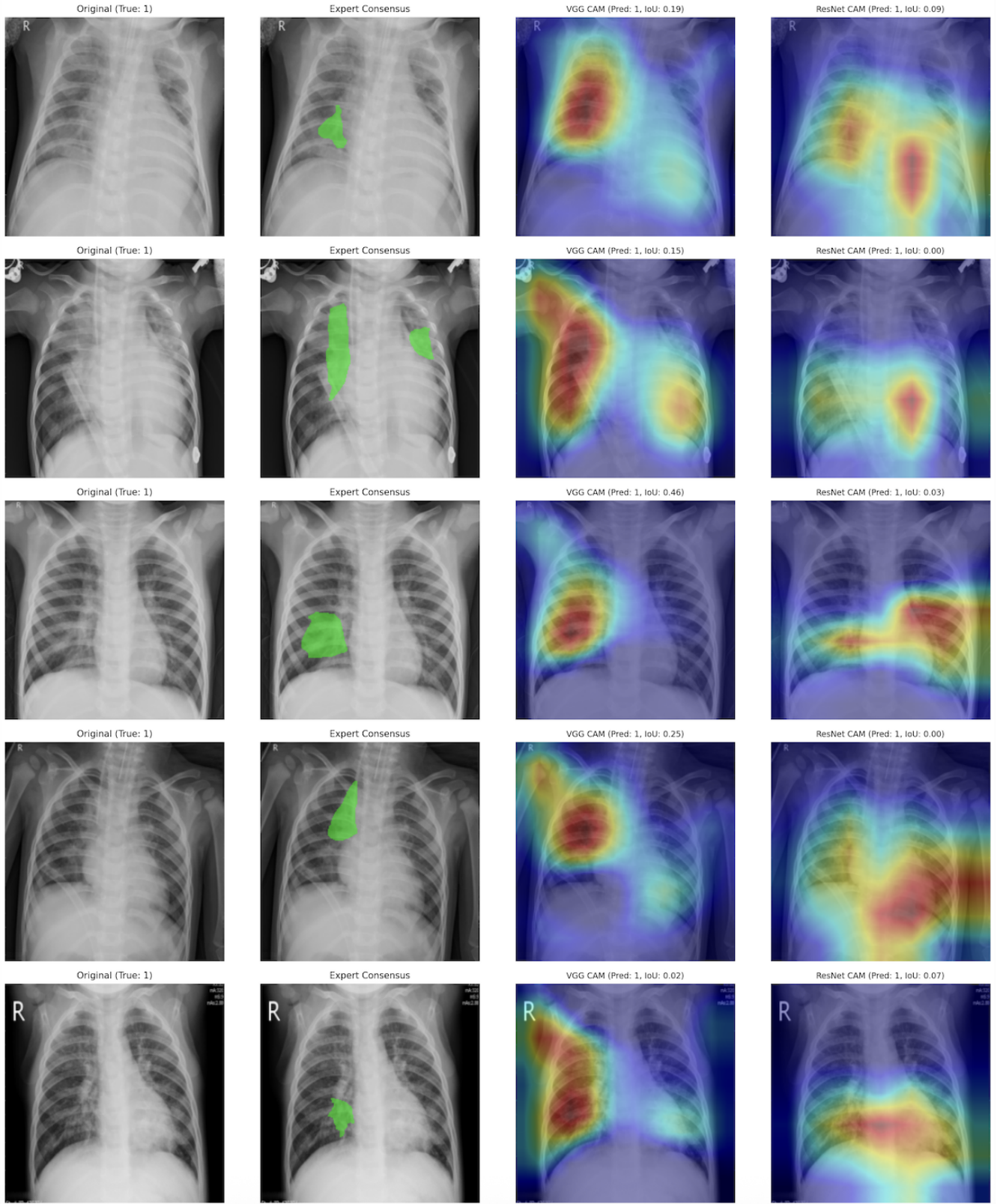
Figure 8: Saliency Map Comparison. Visual comparison between expert annotations and model-generated saliency maps for five pneumonia cases. For each case, from the left: original X-ray, expert consensus annotation (green overlay), VGG-16 CAM, and ResNet-50 CAM.
